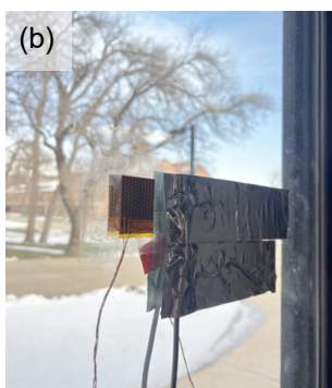
Figure 3. Heat flux field testing method (a) schematic and (b) deployed to measure an IGU on CU Boulder campus
